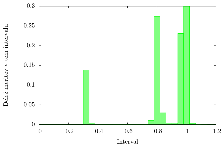
EXAFS
